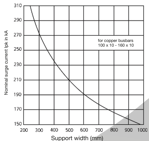
Short-circuit resistance of L185/2
