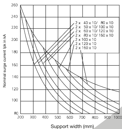
Short-circuit resistance of SH 125
